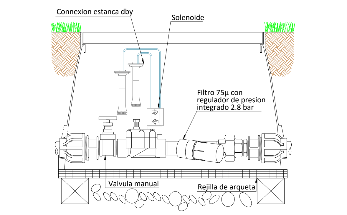
KIT DE CONTROL X CZ-100-PRF / PROG S/E
