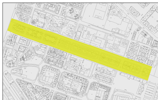
Plano catastral 2009
